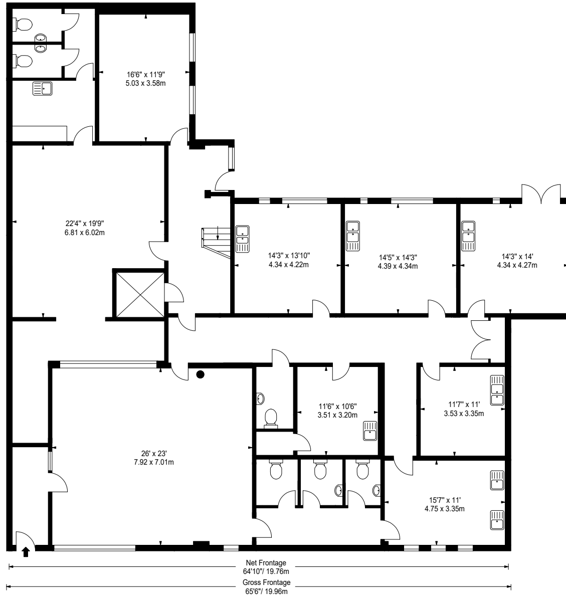
GROUND FLOOR
