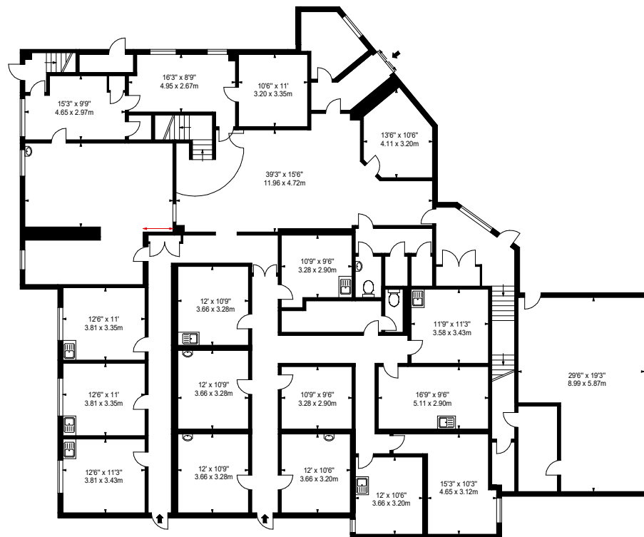
GROUND FLOOR
