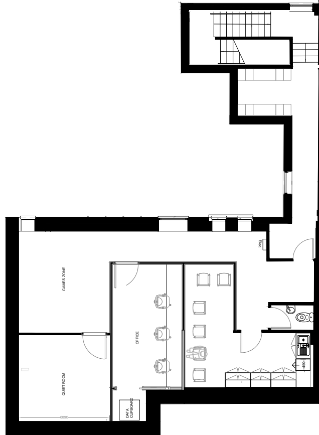
FIRST FLOOR PLAN 1:150
